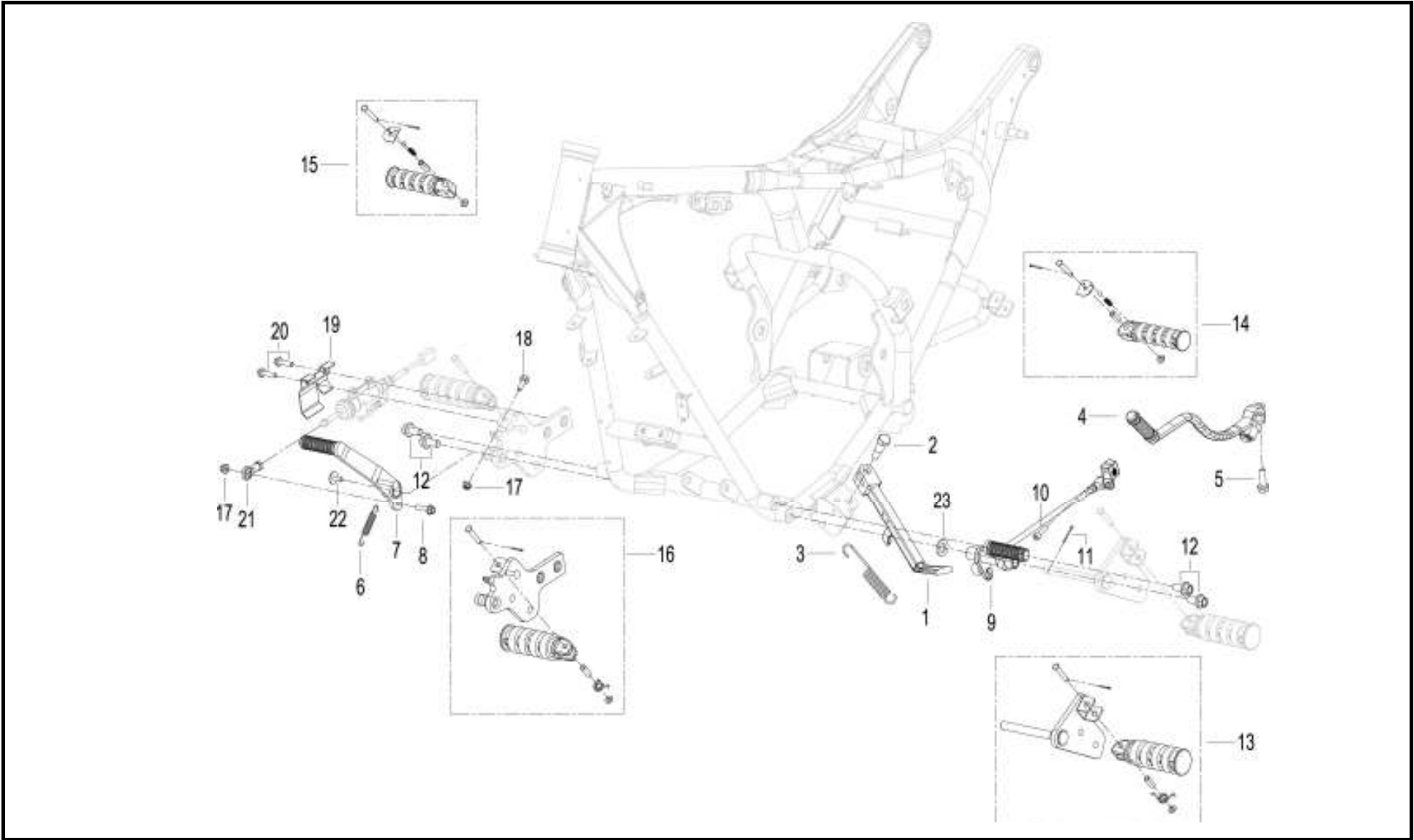
F13 脚蹬 PEDAL ASSY.
