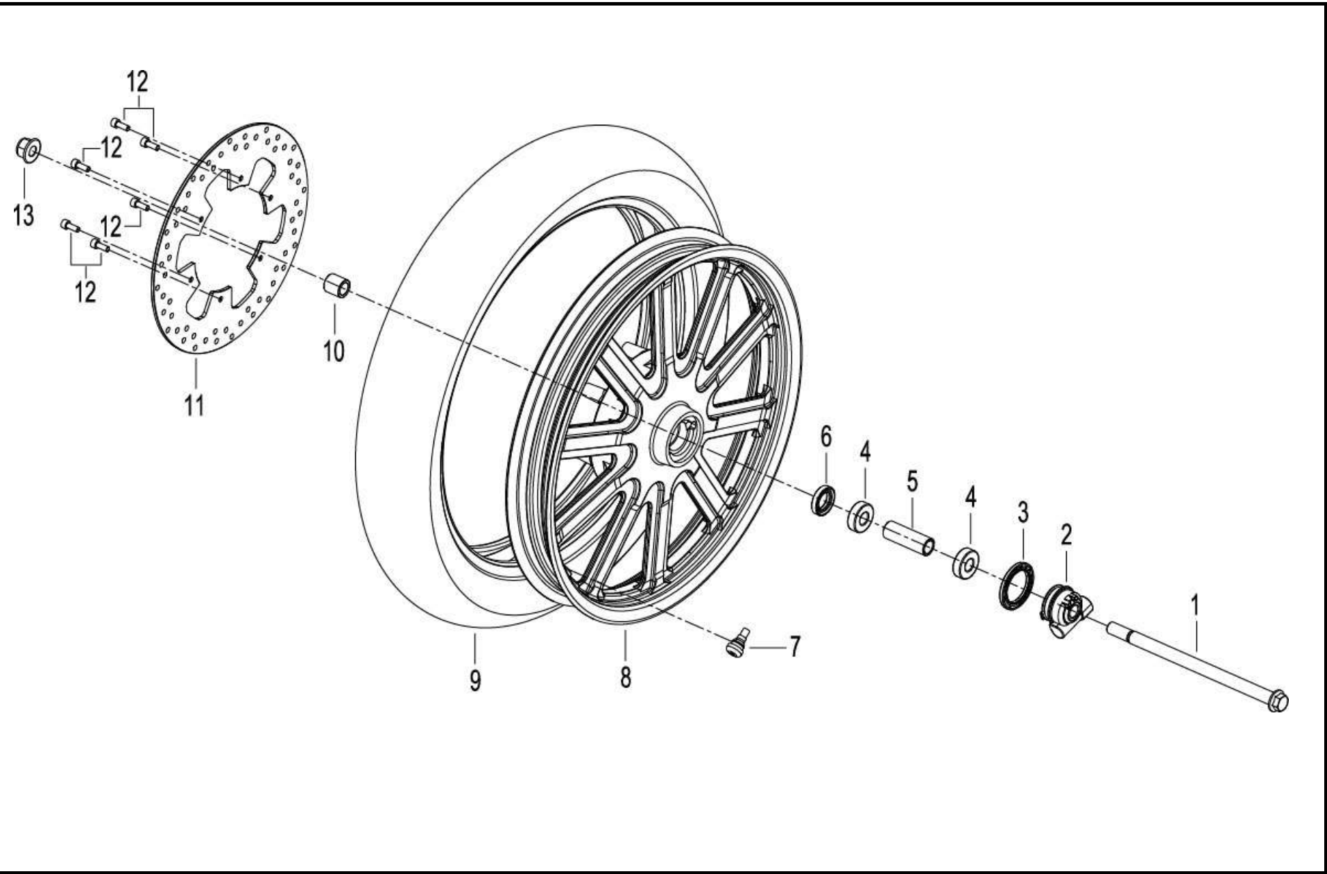
F05 前轮 FRONT WHEEL ASSY.
