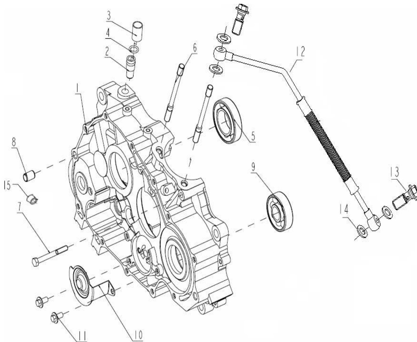
E08.右曲轴箱分总成 RIGHT CRANKCASE ASSY
